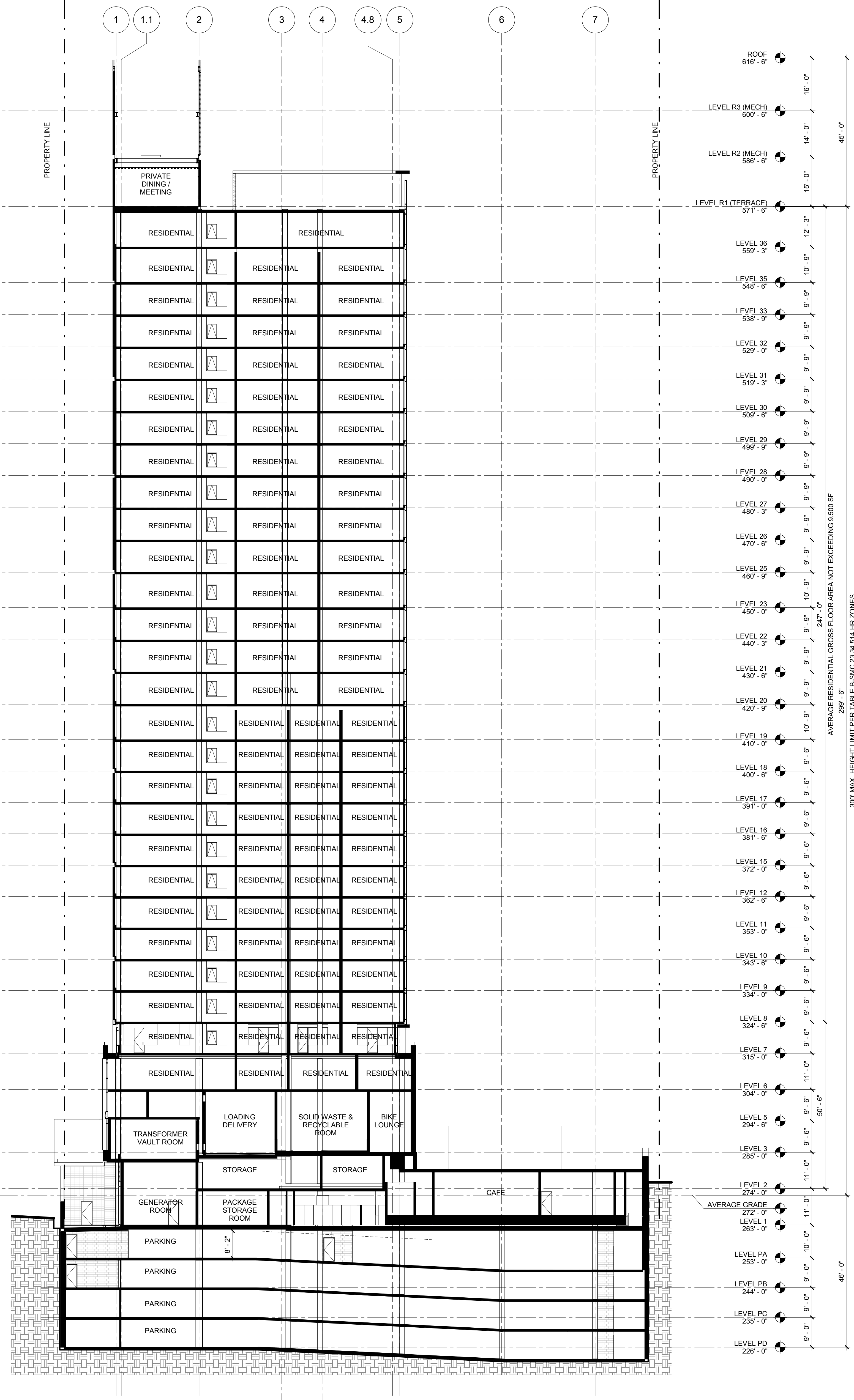
2 NORTH - SOUTH SECTION THRU OPEN SPACE PARK 1/16" = 1'-0"
